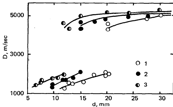
Fig 5 Steady-state detonation velocity of Tetryl ( \rho_0 = 0.9\text{g/cm}^3 ) as a function of charge diameter. Particle size, in mm: 1) 1.0-1.6; 2) 0.63-1.0; 3) 0.4-0.63
